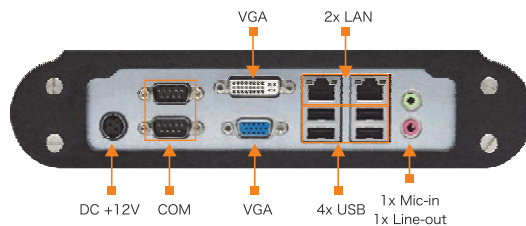
BIS-6650 | BIS-6650B | BIS-6650C接口
